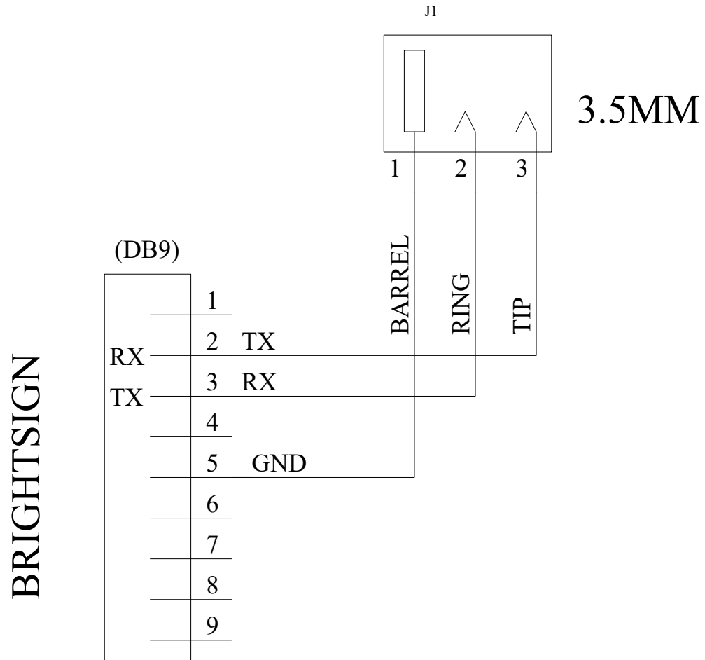
RS232 ADAPTER DB9 TO 3.5MM SCHEMATIC
